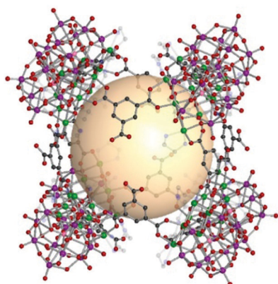
Fig. 16 Structural illustration of [\text{Ni}_6((\text{OCH}_2)_3\text{CNH}_2)(\text{PW}_9\text{O}_{34})_8](\text{B37})_{12} . 82
