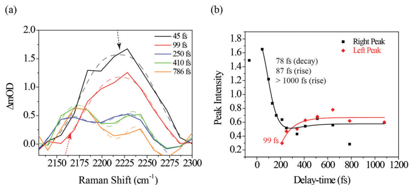
Fig. 7 (a) Closeup of the Raman shift region around 2100–2300 \text{cm}^{-1} where the ODIBO ^5_1\nu_{\text{C}\equiv\text{C}} feature is expected. The spectra at the different time-delays are fit with single and double Gaussians (dotted lines) to describe the peak's change from a single to double-peak feature at \sim 200 fs delay time. (b) Intensity dynamics of the left ( 2165 \text{ cm}^{-1} ) band and right ( 2230 \text{ cm}^{-1} ) band fit with a single and three-component exponential model, respectively (solid curves).
