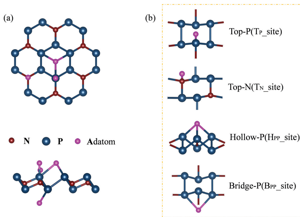
Fig. 3 (a) A schematic illustration of top and side views of the embedded single atom, and (b) adsorption sites of the atoms on monolayer N_2P_6 as presented in Table 1.
