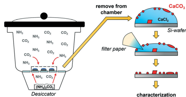
Fig. 1 Schematic view of the droplet-based ammonia diffusion method. Experiments are performed in 20 \mu\text{L} \text{CaCl}_2 droplets on silica wafers. After the reaction is finished, the solvent is quickly removed using a filter paper. The precipitates on the wafer are then dried and investigated.
