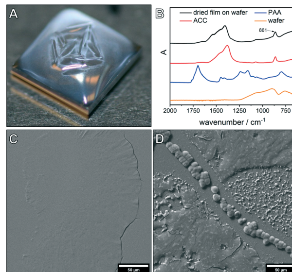
Fig. 2 Characterization of wafers after 1 h gas diffusion experiments with PAA additive. A) The film is visible to the naked eye, here shown for a PAA concentration of 0.5 \text{g L}^{-1} . B) ATR-FTIR spectra show that the precipitates on the wafer are ACC, confirmed by the band at 861 \text{cm}^{-1} , even for the highest additive concentration of 1 \text{g L}^{-1} . For comparison, spectra of pure ACC, pure PAA and the wafer are shown as well. Experimental conditions: 2 h gas diffusion experiment using 20 mM \text{CaCl}_2 solution with 1 \text{g L}^{-1} PAA. C) SEM image of the dried film on the wafer using 10 mM \text{CaCl}_2 and 0.01 \text{g L}^{-1} PAA and D) using 40 mM \text{CaCl}_2 and 0.01 \text{mg L}^{-1} PAA.
