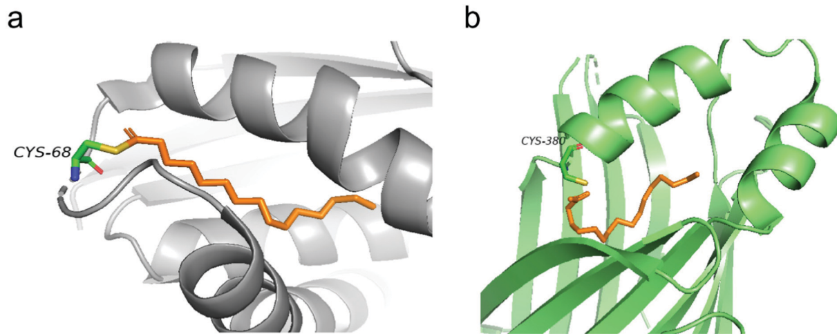
Fig. 2 (a) Palmitate (orange) covalently attaches to C68 in the structure of human Bet3 (PDB code 1S27). (b) Crystal structure of human TEAD2 YBD bound with palmitate (orange) (PDB code 5HG0).
