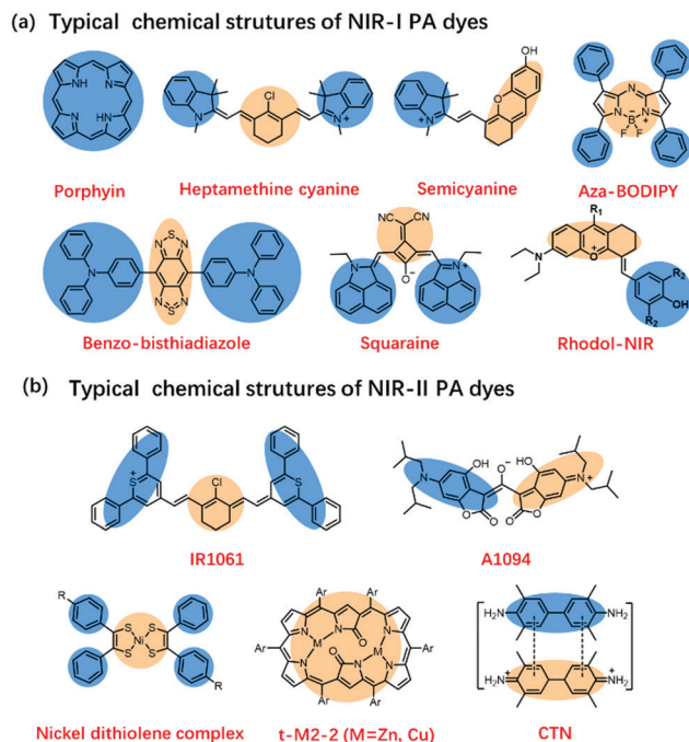
Fig. 2 (a) Typical chemical structures of NIR-I PA dyes. (b) Typical chemical structures of NIR-II PA dyes.
