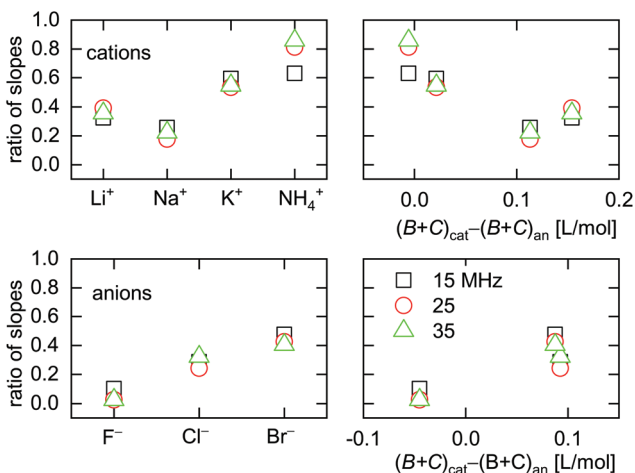
Fig. 9 Ratio of slopes \langle A/\Delta E \rangle_{\Delta f} / (-\langle A/\Delta E \rangle_{\Delta \Gamma}) as obtained from \Delta \Gamma and \Delta f (eqn (13)). Large ratios indicate a large elastic contribution. \text{Cs}^+ was omitted from this graph because the sign of \langle A/\Delta E \rangle_{\Delta \Gamma} for \text{Cs}^+ was opposite to the sign of \langle A/\Delta E \rangle_{\Delta f} for all other ions.
