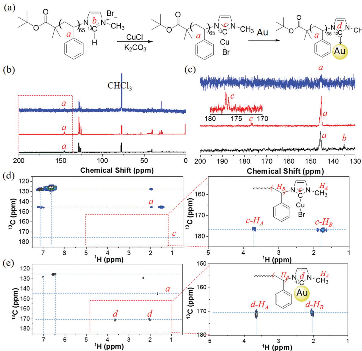
Fig. 3 (a) Synthesis of ^{13}\text{C} -labeled \text{PS}_{65}\text{-}^{13}\text{C-NHC-Au} using ^{13}\text{C} -Im. (b and c) ^{13}\text{C} NMR spectra of \text{PS}_{65}\text{-}^{13}\text{C-NHC-Im} (black, bottom), \text{PS}_{65}\text{-}^{13}\text{C-NHC-Cu(I)} (red, middle) and \text{PS}_{65}\text{-}^{13}\text{C-NHC-Au} (blue, top) in \text{CDCl}_3 . ^{13}\text{C} NMR spectra in (b) in the range of 130–200 ppm is zoomed in (c). (d) 2D HMBC spectrum of non-labeled \text{PS}_{65}\text{-NHC-Cu(I)} . (e) 2D HMBC spectrum of ^{13}\text{C} -labeled \text{PS}_{65}\text{-}^{13}\text{CNHC-Au} .
