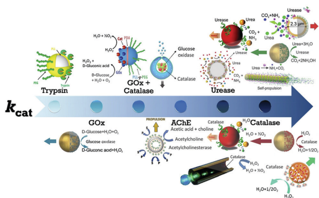
Fig. 3 Schematic of enzymes reported to power micro/nanomotors (MNMs) arranged in an ascending order of turnover number ( k_{\text{cat}} ): trypsin, 113 glucose oxidase (GOx), 114 GOx coupled with catalase, 115,116 acetylcholinesterase (AChE), 117 urease, 20,70,114,118 and catalase. 18,69,114,119 Adapted with permission from ref. 20, 69, 113–116 and 118 and 119. Copyrights 2010, 2015, 2016, and 2017 American Chemical Society. Adapted with permission from ref. 117. Copyright 2019 Springer Nature. Adapted with permission from ref. 70. Copyright 2018 Wiley. Adapted with permission from ref. 18. Copyright 2017 Elsevier.
