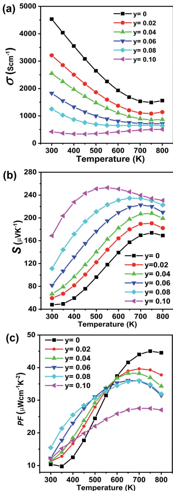
Fig. 10 Electronic transport properties as a function of temperature for Ge 0.97-y Cd 0.03 Sb y Te ( y = 0-0.10 ) samples: (a) electrical conductivity and (b) Seebeck coefficient. The increasing and decreasing trends in the electrical conductivity and the Seebeck coefficient at high temperatures indicate the presence of bipolar conduction. (c) Power factor as a function of temperature for Ge 0.97-y Cd 0.03 Sb y Te ( y = 0-0.10 ) samples, showing a large enhancement at temperatures below 600 K with respect to the sample with no Sb doping.
