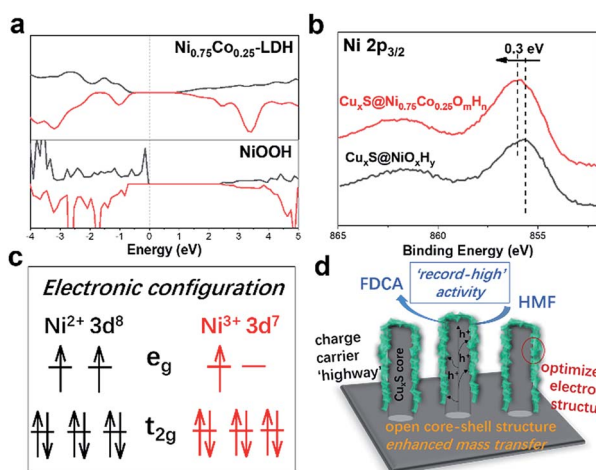
Fig. 4 (a) Projected density of states calculations for Ni_{0.75}Co_{0.25} -LDH and NiOOH. (b) High resolution Ni 2p 3/2 XPS spectra of \text{Cu}_x\text{S}@Ni_{0.75}Co_{0.25}O_mH_n and \text{Cu}_x\text{S}@NiO_mH_n . (c) Schematic illustration of the electronic configuration of the Ni cations with valence states of +2 and +3. (d) Schematic illustration of factors contributing to the high HMF oxidation activity.
