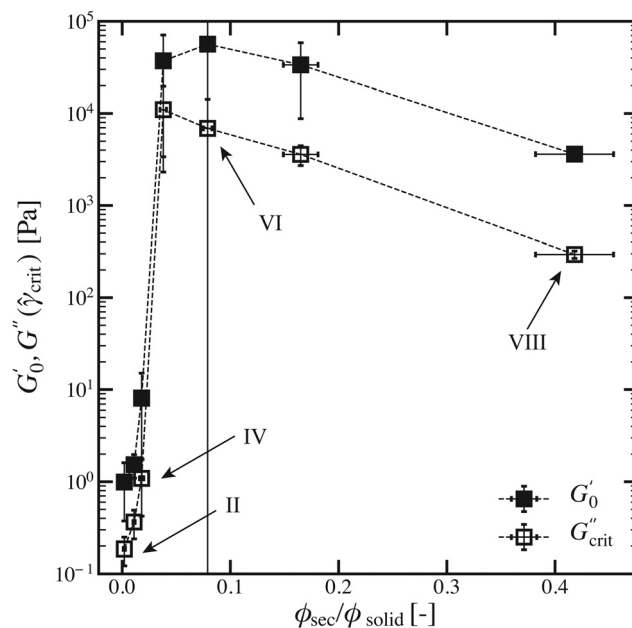
Fig. 9 Plateau storage modulus G_0' and loss modulus value G''(\dot{\gamma}_{crit}) at the end of the LVE region, as function of the effective secondary fluid to solid volume ratio \phi_{sec}/\phi_{solid} for the samples with particles having \theta = 87^\circ \pm 8^\circ . The frequency was fixed at \omega = 10 \text{ rad s}^{-1} .
