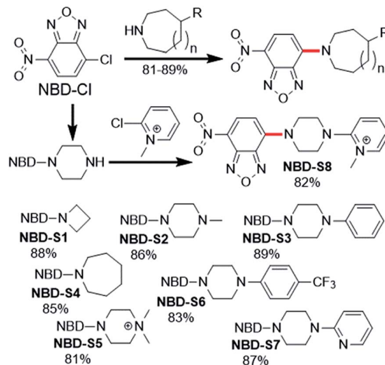
Fig. 2 Synthesis of NBD amines NBD-S1 to NBD-S8 . The C–N bond cleaved by \text{H}_2\text{S} -mediated thiolysis is highlighted in red in each structure.
