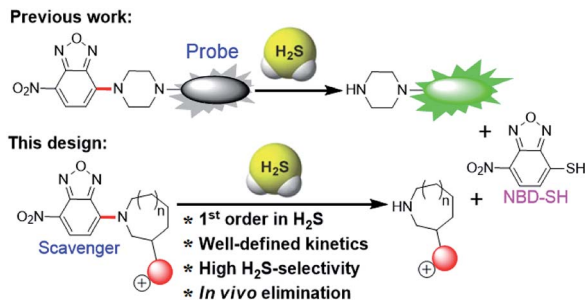
Fig. 1 (top) The thiolysis of NBD amines used previously for \text{H}_2\text{S} probe development. (bottom) Inclusion of cationic charge in the present system enables access to efficient \text{H}_2\text{S} scavengers by thiolysis of NBD cyclic amines.
