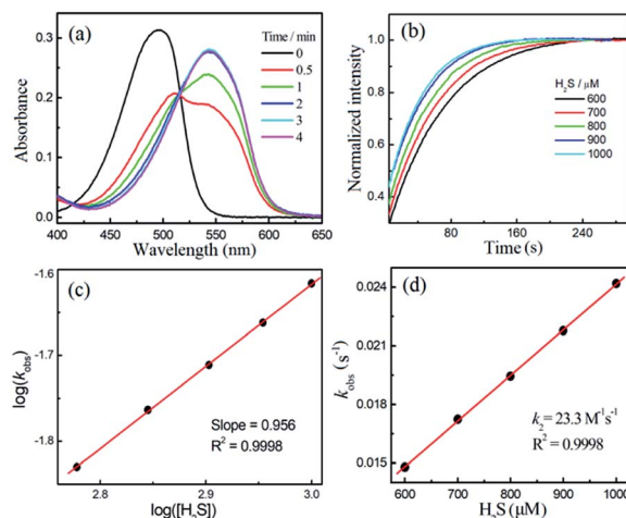
Fig. 3 (a) Time-dependent absorbance spectra of 10 \mu\text{M} NBD-S2 towards 1 mM \text{H}_2\text{S} in PBS buffer (50 mM, pH = 7.4, containing 2% DMSO) at 25 ^\circ\text{C} . (b) Time-dependent normalized signals at 540 nm of 10 \mu\text{M} NBD-S2 towards different concentrations of \text{H}_2\text{S} . (c) The reaction order of \text{H}_2\text{S} was determined as the slope of plots of \log(k_{\text{obs}}) versus \log([\text{H}_2\text{S}]) . (d) The k_2 was determined as the slope of plots of k_{\text{obs}} versus [\text{H}_2\text{S}] .
