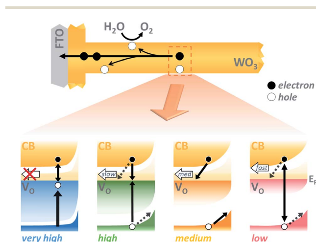
Scheme 1 (Upper) Illustration of a single nanoneedle of WO_3 (yellow) on FTO (grey), indicating electron (black) transport (black arrows) and possible recombination pathways with holes (white) on route to extraction. (Lower) Indication of the dominant kinetic pathways immediately following charge separation in each of the samples examined: ‘very high’ [ V_O ] (left, blue), ‘high’ [ V_O ] (centre left, green), ‘medium’ [ V_O ] (centre right, yellow) and ‘low’ [ V_O ] (right, red). Arrow weight depicts likelihood of event. Filled V_O states are given in colour, empty states able to trap electrons are given in yellow. ‘Very high’ [ V_O ] shows hole trapping faster than instrument detection (heavy arrow). The ‘high’ doped sample has the greatest bulk trap recombination, particularly from hole trapping, so later carrier collection is limited. With too few defect states (‘low’, red), charge separation is hindered and the probability of geminate and bimolecular recombination increases. The best performing sample has the optimal amount of defects to aid charge separation without losing carriers to trap-mediated recombination.
