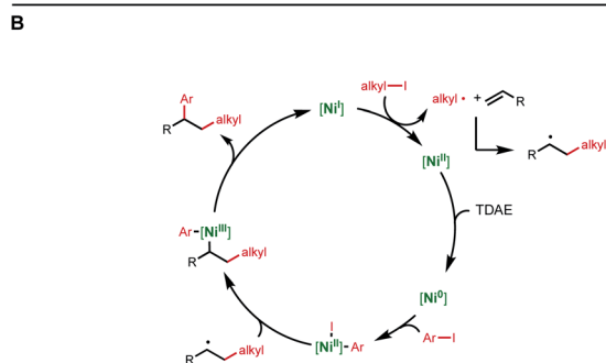
Fig. 2 (A) Reductive 1,2-dicarbofunctionalization of acrylate-type compounds. (B) Proposed catalytic cycle.
