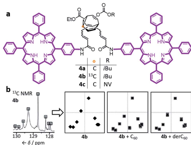
Fig. 4 (a) Bode's bisporphyrin-bullvalene 4, which was prepared with natural isotopic abundance (4a), enriched in ^{13}\text{C} at one position (4b) of the dynamic C 10 core, and functionalised with a photocleavable group (4c). (b) The complex ^{13}\text{C} NMR spectra of the dynamic mixtures are converted to simplified representations, showing that the ^{13}\text{C} NMR spectrum of a 4b mixture at equilibrium changes in the presence of fullerene guests. NMR data (150 MHz, solutions in CS 2 with 3% CD 2 Cl 2 ) shown for samples of: (4b) 2.8 mM 4b; (4b + C 60 ) 2.8 mM 4b with 2 equiv. C 60 ; (4b + derC 60 ) 2.8 mM 4b with 4 equiv. derC 60 . The representations of NMR spectra correspond to two trials overlaid. NV = o-nitroveratryl. Adapted from ref. 7e with permission from The Royal Society of Chemistry.
