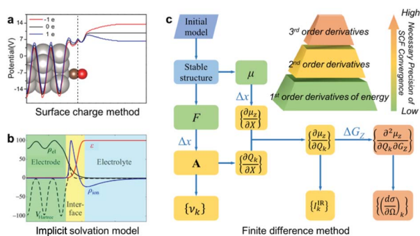
Scheme 1 The computational method for EC-IR and EC-Raman spectra: (a) surface charged method, (b) implicit solvation model and (c) finite difference method. \mu , F , X , A , \nu_k and G_Z represent the surface dipole moment, atomic force, external atomic coordinates, dynamical matrix at the T point, vibrational frequency of the k^{\text{th}} normal-mode coordinate Q_k , and external electric field along the Z axis, respectively. \Delta x and \Delta G_Z represent the step size of X and G_Z for the finite difference. Image (a) adapted from ref. 38 with permission, copyright (2011) Royal Society of Chemistry; image (b) adapted from ref. 29 with permission, copyright (2014) American Institute of Physics.
