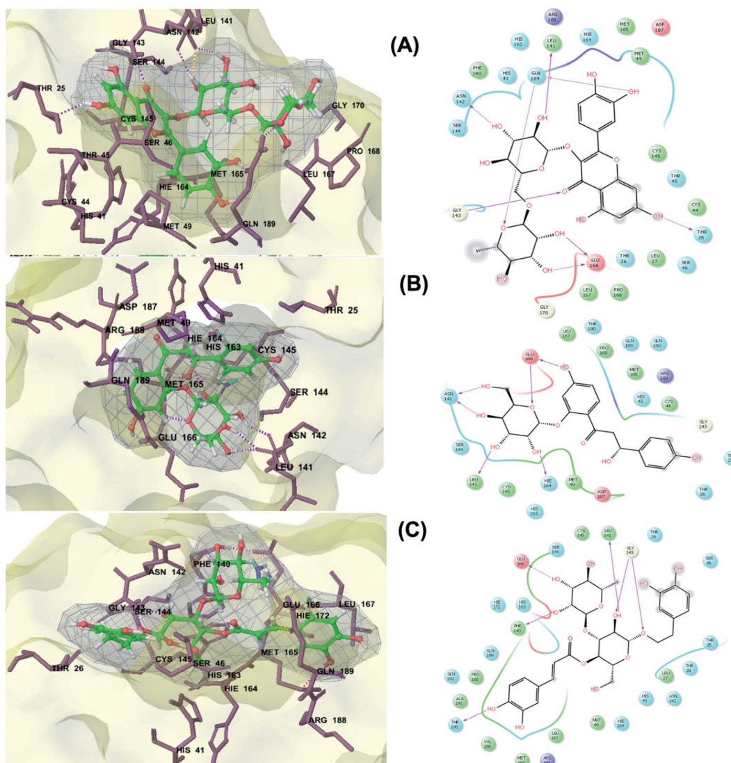
Fig. 1 3D (to the left) and 2D (to the right) interaction diagrams of (A) rutin, (B) rocymsin b and (C) verbasoside with the crystal structure of 3CLpro (PDB ID: 5R7Y).
