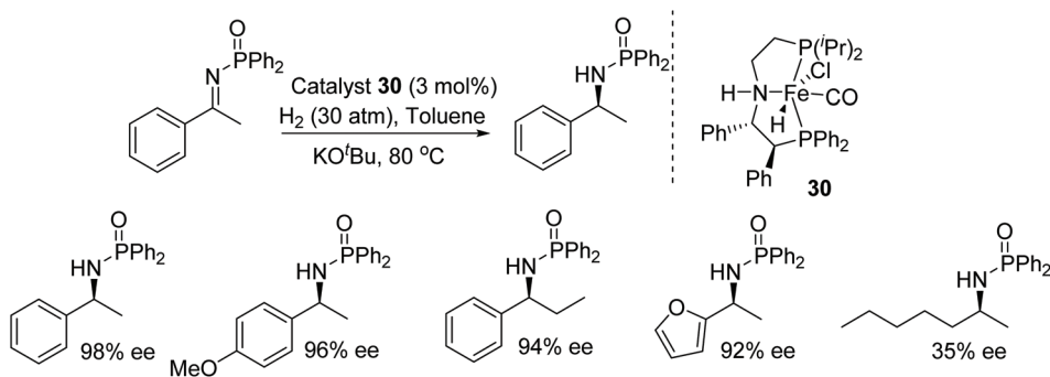
Fig. 41 Iron catalyzed AH of activated imines.
