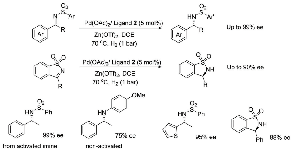
Fig. 39 Palladium catalyzed AH of sulfonfylimines.
