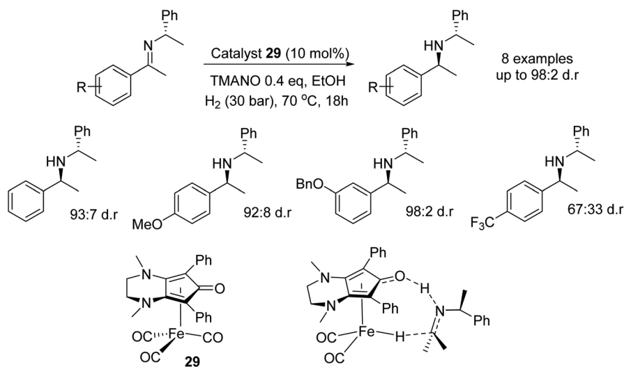
Fig. 40 Iron catalyzed diastereoselective hydrogenation of N -alkylated chiral imines.
