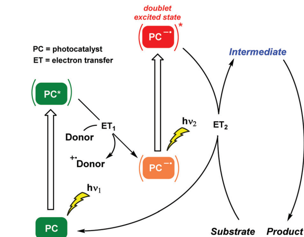
Scheme 6 The ConPET mechanism, which mimics the Z-scheme, adapted to organic transformations. Selective excitation of the PC led to its excited state which is quenched by an appropriate donor generating the PC radical anion. Then, excitation of the PC radical anion results in the formation of an excited PC radical anion (doublet excited state), a highly reducing agent.
