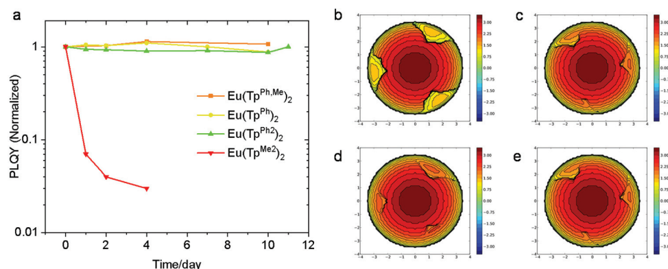
Fig. 3 (a) The normalized PLQY changes of crystalline \text{Eu}(\text{Tp}^{\text{Me2}})_2 , \text{Eu}(\text{Tp}^{\text{Ph,Me}})_2 , \text{Eu}(\text{Tp}^{\text{Ph}})_2 and \text{Eu}(\text{Tp}^{\text{Ph2}})_2 in air. Topographic steric maps of \text{Eu}(\text{Tp}^{\text{Me2}})_2 (b), \text{Eu}(\text{Tp}^{\text{Ph,Me}})_2 (c), \text{Eu}(\text{Tp}^{\text{Ph}})_2 (d) and \text{Eu}(\text{Tp}^{\text{Ph2}})_2 (e). Red and blue indicate the more- and less-hindered zones, respectively. 29
