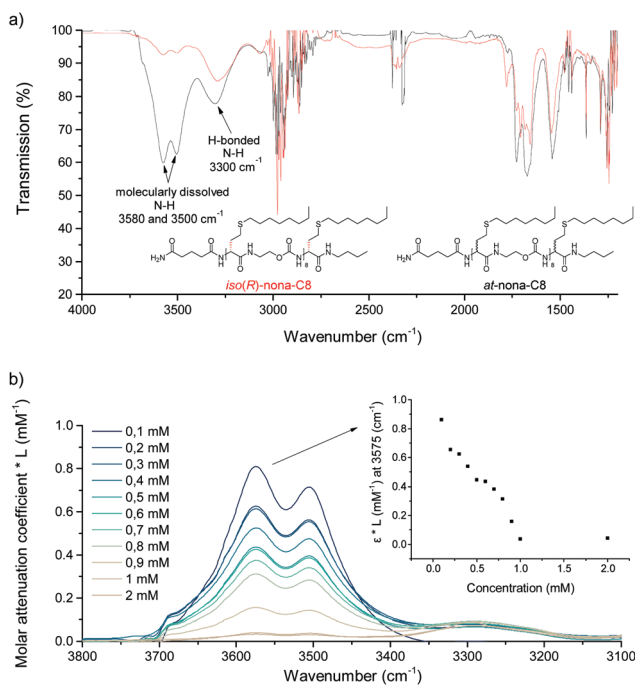
Fig. 6 (a) Comparison of IR-absorption iso(R) -nona-C8 and at -nona-C8, whereby two different N -H stretches are indicated. (b) Molar attenuation coefficient of iso(R) -nona-C8 at different concentration and at 3575 cm -1 .
