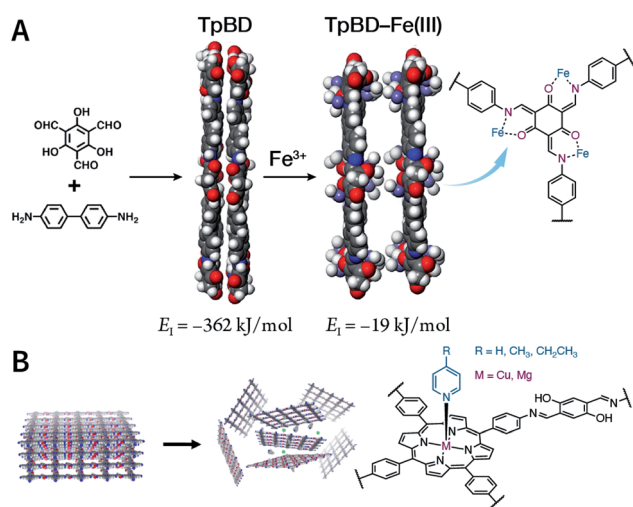
Fig. 20 Coordination-induced chemical exfoliation of COFs. (A) Fe 3+ -assisted aqueous-phase chemical exfoliation to prepare TpBD COF nanosheets. Adapted under a Creative Commons Attribution 4.0 International License. Copyright 2018, The Author(s). 175 Published by Springer Nature Limited. (B) Porphyrin-based nanodisks synthesized via the simultaneous axial coordination of pyridines and metal ions. Adapted under a Creative Commons Attribution 4.0 International License. Copyright 2019, The Author(s). 176 Published by Springer Nature Limited.
