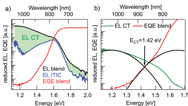
Fig. 4 Determination of CT state energy. (a) Reduced EQE \times E spectrum for an inverted BHJ solar cell (red) together with EL/E spectra for the same solar cell (black trace) and an ITIC diode (blue). The green shaded area represents the CT EL emission. (b) Subtracted solar cell EL/E spectrum (green) and reduced EQE \times E spectrum (red) together with Gaussian fitting curves (black) to determine E_{CT} .
