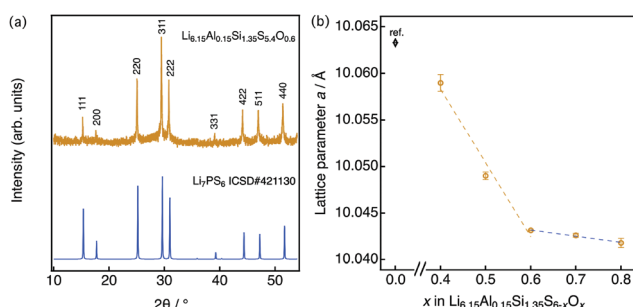
Fig. 2 (a) X-ray diffraction pattern for \text{Li}_{6.15}\text{Al}_{0.15}\text{Si}_{1.35}\text{S}_{5.4}\text{O}_{0.6} along with the pattern of argyrodite \text{Li}_7\text{PS}_6 (ICSD#421130), which is indexed as the cubic argyrodite phase. (b) Lattice parameter for \text{Li}_{6.15}\text{Al}_{0.15}\text{Si}_{1.35}\text{S}_{6-x}\text{O}_x as a function of the nominal oxygen content x . The lattice data for x = 0 are taken from the literature. 25
