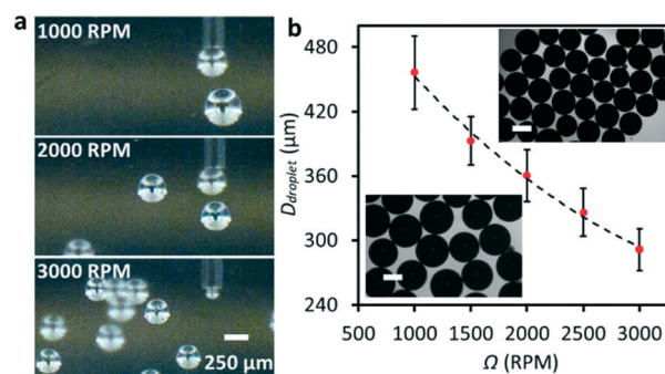
Fig. 4 Production of EGaIn microdroplets using the RNEG. a) Images taken from a high-speed camera showing the production of liquid metal microdroplets at different revolving speeds. b) Plot of the droplet diameter D_{\text{droplet}} vs. \Omega . The inset images show the EGaIn droplets produced when \Omega is 1500 and 3000 rpm, respectively, and Q is 20 \mu\text{L min}^{-1} .
