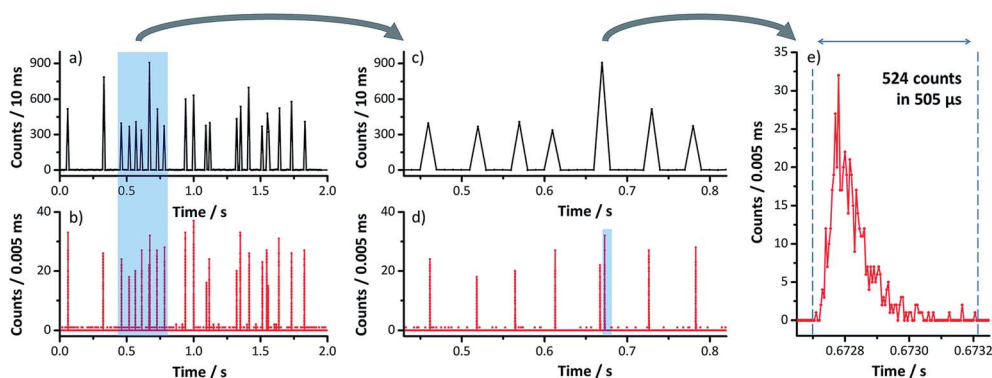
Fig. 6 Representative ICP-MS signal (monitoring m/z 197 \text{Au}^+ ) due to 30 nm Au NPs ( C_{\text{NP}} = 2.5 \times 10^5 \text{ NP mL}^{-1} ) acquired simultaneously for 2 s with (a) 10 ms dwell time (vendor software), and (b) 5 \mu s dwell time (home-built data acquisition system). First zoom level shows several particle events in (c) and (d) for 500 ms (of the highlighted section in a and b). Second zoom level (e) shows the temporal profile of a single particle's ion cloud identified with the home-built data acquisition system in (d). Reproduced from Strengé and Engelhard 77 with permission from the Royal Society of Chemistry.
