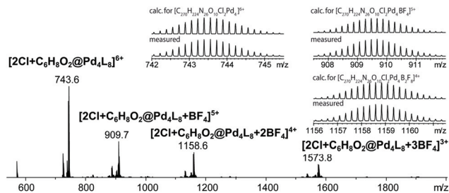
Fig. 4 ESI-MS spectrum of the host-guest complex [2\text{Cl} + \text{C}_6\text{H}_8\text{O}_2@\text{Pd}_4\text{L}_8] obtained by the slow photosensitization of a cage-substrate mixture in the presence of air after 94 days.
