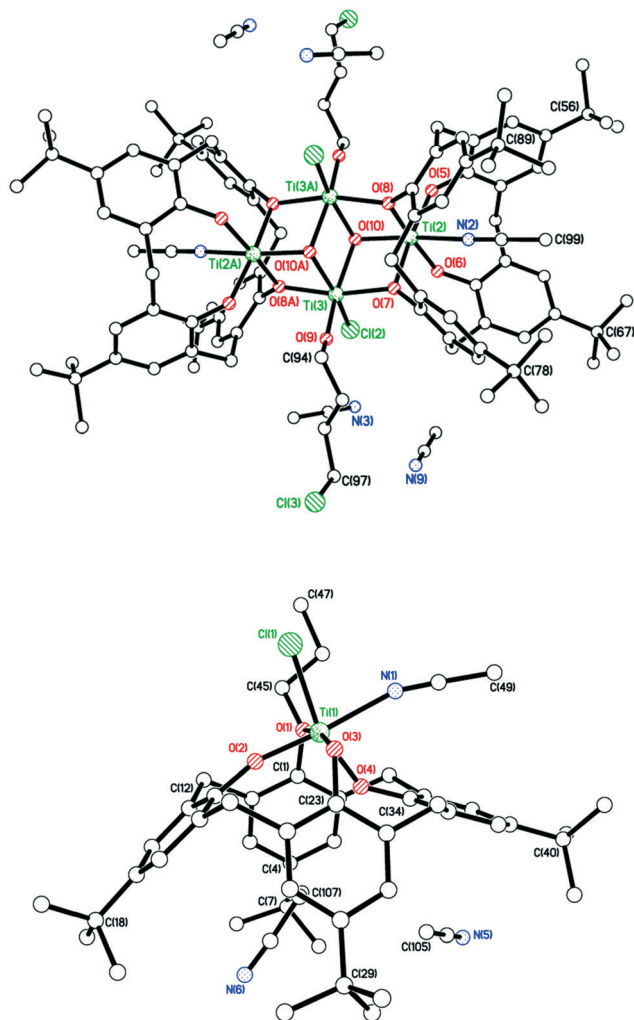
Fig. 6 Molecular structure of [\text{Ti}(\text{NCMe})(\mu_3\text{-O})(\text{L})_4\text{TiCl}(\text{O}(\text{CH}_2)_4\text{Cl})]_2 \cdot 2[\text{TiCl}(\text{NCMe})(\text{L})(\text{O})_3(\text{On-Pr})] \cdot 11\text{MeCN} (8·11MeCN) (H atoms and some solvent molecules are omitted for clarity). Selected bond lengths (Å) and angles ( ^\circ ): Ti(1)–O(1) 2.3307(19), Ti(1)–O(2) 1.7892(19), Ti(1)–O(3) 1.8406(18), Ti(1)–O(4) 1.8534(19), Ti(1)–N(1) 2.234(2), Ti(1)–Cl(1) 2.3363(8), Ti(2)–O(5) 1.8362(17), Ti(2)–O(6) 1.8321(17), Ti(2)–O(7) 2.0607(16), Ti(2)–O(8) 2.0497(16), Ti(2)–O(10) 1.8463(17), Ti(2)–N(2) 2.207(2), Ti(3)–O(7) 1.9800(17), Ti(3)–O(9) 1.855(2), Ti(3)–O(10) 2.0834(17), Ti(3)–O(8A) 2.0216(17), Ti(3)–O(10A) 2.0139(17), Ti(3)–Cl(2) 2.2999(7); O(1)–Ti(1)–O(3) 168.80(8), O(2)–Ti(1)–O(4) 102.23(9), Ti(1)–O(1)–C(1) 115.47(15), Ti(1)–O(2)–C(12) 162.29(19), Ti(1)–O(3)–C(23) 120.39(15), Ti(1)–O(4)–C(34) 142.39(16).
