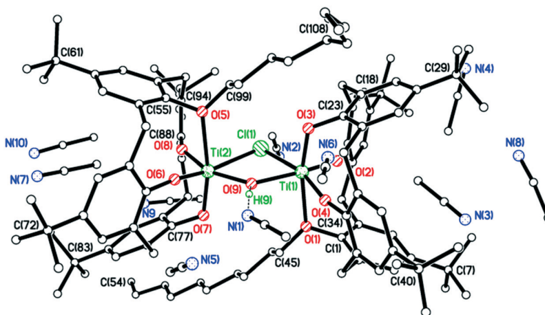
Fig. 7 Molecular structure of \{[\text{TiL}(\text{O})_3(\text{On-decyl})]_2(\mu\text{-Cl})(\mu\text{-OH})\} \cdot 8.5\text{MeCN} ( 10 · 8.5MeCN ) (most H atoms are omitted for clarity). Selected bond lengths (Å) and angles (°): Ti(1)–O(1) 2.381(3), Ti(1)–O(2) 1.817(3), Ti(1)–O(3) 1.852(3), Ti(1)–O(4) 1.793(3), Ti(1)–O(9) 2.000(3), Ti(1)–Cl(1) 2.5177(14); O(1)–Ti(1)–O(3) 168.54(13), O(2)–Ti(1)–O(4) 102.84(15), Cl(1)–Ti(1)–O(9) 74.82(10), Ti(1)–O(1)–C(1) 112.8(2), Ti(1)–O(2)–C(12) 150.5(3), Ti(1)–O(3)–C(23) 119.9(2), Ti(1)–O(4)–C(34) 168.3(3).
