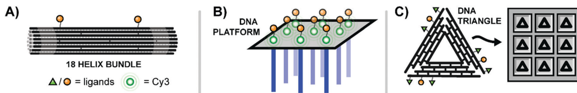
Fig. 13 Multivalent binding agents constructed using DNA origami. (A) 18-Bundle helix origami provides a rigid platform for bivalent ligands targeting Ephrin receptors (ref. 42). (B) Rectangular DNA origami platform with dangling strands for hybridization to nanoarray (blue) and Cy3-EGF ligands for receptor binding (green) (ref. 43). (C) Triangular DNA origami platforms decorated with ligands for EGFR and \beta 6 integrin are loaded into etched wells to create a surface with finely-tunable ligand patterning (ref. 44).
