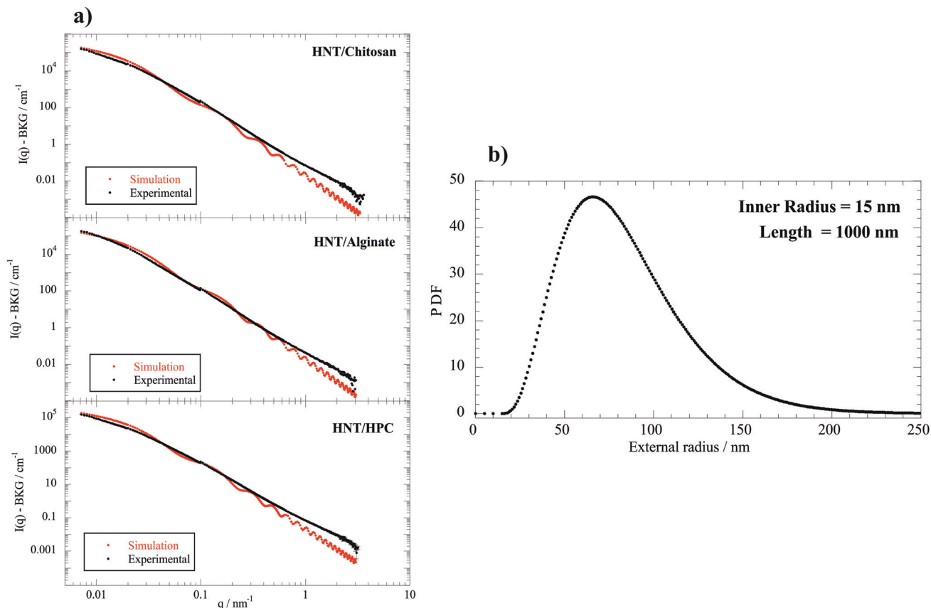
Fig. 3 (a) SANS intensity as a function of q , the magnitude of the scattering vector, after background subtraction for HNT/alginate, HNT/chitosan and HNT/HPC dispersions in \text{D}_2\text{O} . The best simulation results (red points) were obtained according to a hollow cylinder as model (eqn (8)) with fixed length (1000 nm) and inner radius (15 nm). (b) Schulz-Zimm distribution for the external radius was centered at 65 nm. The incoherent scattered background was evaluated by Porod analysis applied to the larger q range.
