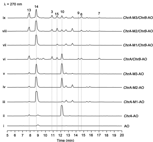
Fig. 5 Co-expression of KR-mutated ChrA and ChrB in A. oryzae (AO). HPLC traces for metabolites produced by AO ((i), as a blank reference), the transformants [with ChrA (ii), ChrA -M1 for K^{1829}D (iii), ChrA -M2 for S^{1853}A (iv), and ChrA -M3 for Y^{1866}A (v)], and the co-transformants with ChrA and ChrB (vi), ChrA -M1 and ChrB (vii), ChrA -M2 and ChrB (viii), and ChrA -M3 and ChrB (ix).
