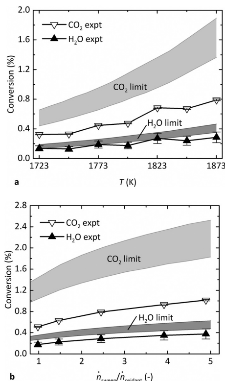
Fig. 4 Comparison of the average experimental conversion of \text{CO}_2 and \text{H}_2\text{O} at steady state versus equilibrium limits as a function of (a) T , at \dot{n}_{\text{sweep}}/\dot{n}_{\text{oxidant}} = 2.4 and 1 Pa \text{O}_2 , and (b) \dot{n}_{\text{sweep}}/\dot{n}_{\text{oxidant}} , at 1873 K and 0.5 Pa \text{O}_2 .
