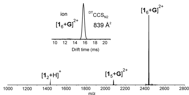
Fig. 1 (+)ESI-MS spectrum of 1 (60 \mu M) and tris(bipyridine)ruthenium(II) ( G ) with 6 : 1 ratio measured from acetone/DCM mixture. Inset showing IMS arrival time distribution (ATD) for [ 1 _6 + G ] ^{2+} ion.
