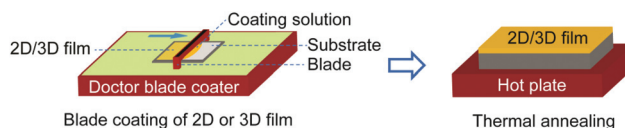
Fig. 1 Schematic illustration of the doctor-blade setup used for the deposition of the 2D PEA 2 PbI 4 and reference 3D FAPbI 3 perovskite films.
