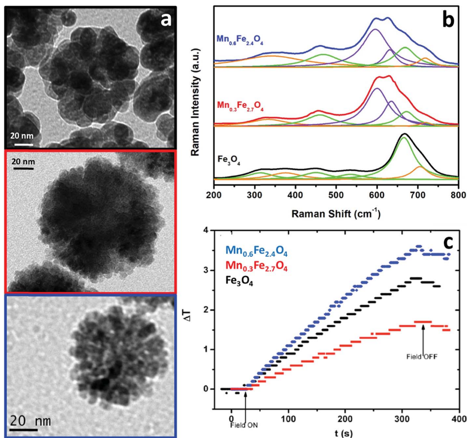
Fig. 7 TEM images (a), Raman spectra (b) and temperature profile during the application of an alternating magnetic field (c) of clusters of Fe_3O_4 , Mn_{0.3}Fe_{2.7}O_4 and Mn_{0.6}Fe_{2.4}O_4 nanoparticles.
