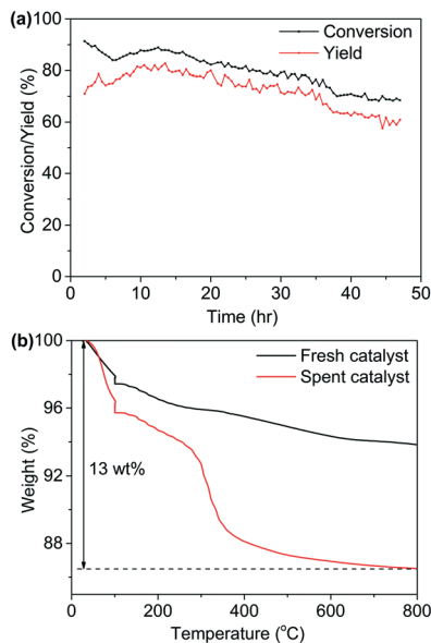
Fig. 6 (a) Stability test for Ni/Al 2 O 3 -PD catalyst. 1-Hexanol at 1 μL min -1 with 8 mL min -1 NH 3 and 20 mL min -1 N 2 flowed through 200 mg catalyst at 230 °C. GHSV = 1.12 × 10 4 h -1 . (b) TG analysis for Ni/Al 2 O 3 -DP catalyst before and after reaction.
