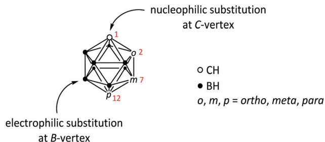
Fig. 1 General structure of icosahedral carboranes of type \text{closo-C}_2\text{B}_{10}\text{H}_{12} . Numbers in red indicate the numbering of the C-vertices of the cluster in the respective isomer: 1,2 ( ortho , o), 1,7 ( meta , m) and 1,12 ( para , p). For detailed explanation of the numbering system in carborane clusters see ref. 1. The two most common types of substitution reactions (nucleophilic at C- and electrophilic at B-vertices) are indicated.
