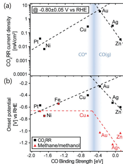
Fig. 16 (a) Volcano plot of partial current density for the e-CO 2 RR assessed at -0.80 \pm 0.05 V vs RHE. (b) Distinct onset potentials plotted vs. CO binding energy for the overall e-CO 2 RR, and for methane/methanol production. Dashed lines serve as a guide. Reprinted with permission from ref. 245. Copyright 2014 American Chemical Society.
