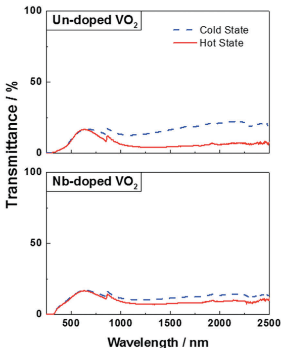
Fig. 9 UV-Vis spectra of un-doped \text{VO}_2 (top) and Nb-doped \text{VO}_2 (bottom) at 20 °C (blue dashed line) and 90 °C (continuous red line).
