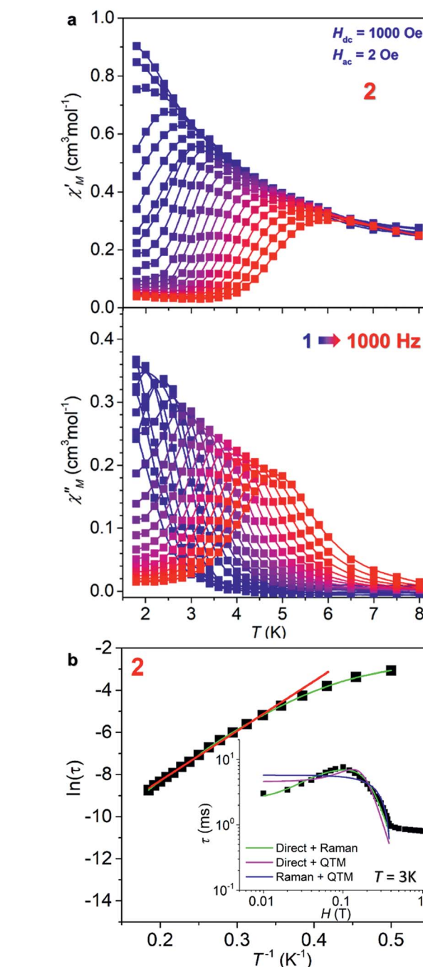
Fig. 4 (a) The in-phase ( \chi' ) and out-of-phase ( \chi'' ) components of the ac susceptibilities as a function of T of 2 in 1000 Oe dc field at different time frequencies (1–1000 Hz). (b) Natural logarithm of the relaxation time \ln \tau as a function of the inverse temperature T^{-1} . The straight red line is a fit of the 12 points at highest temperatures to the Arrhenius law \ln \tau = \ln \tau_0 + U_{\text{eff}}/k_B T . The curved green line is the best fit to the sum of the direct and Raman processes (see ESI†). Inset: field dependence of the magnetic relaxation times at 3 K for 2 and its approximation by the different models assuming two magnetic relaxation mechanisms, where only the sum of the direct and Raman processes gives a good fit.
