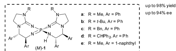
Scheme 1 Catalytic enantioselective direct Mannich-type reactions of 2-alkylazaarene N-oxides.
