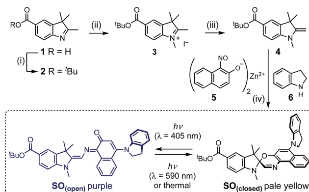
Scheme 1 Synthesis of switch SO . (i) tert -Butyl 2,2,2-trichloroacetimidate, \text{BF}_3\text{OEt}_2 , THF, 20 °C, 20 min, 64%. (ii) MeI, o -DCB, 80 °C, 24 h, 77%. (iii) KOH, 20 °C, 2 h, 99%. (iv) 5 , 6 , EtOH, air, reflux 2 h, then 4 , \text{Na}_2\text{SO}_4 , reflux 21 h, 22%. The photo-switching mechanism of SO is shown.
