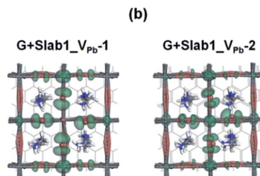
Fig. 13 (a) Calculated partial density of states (PDOS) of MAPbI_3 in the V_{Pb} -containing graphene + MAPbI_3 hybrids, and (b) the orbital shape of the valence band edges of MAPbI_3 (isovalue: 0.015 a.u.).
