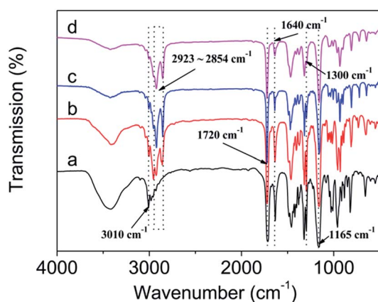
Fig. 3 FTIR spectra of DM-EB (a), DM-HB (b), DM-DB (c) and DM-LB (d).
