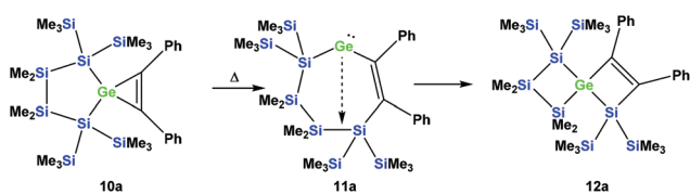
Scheme 6 Expected thermally-induced reaction pathway of 10a to give [3.3]-spirocyclic vinylgermane 12a .
