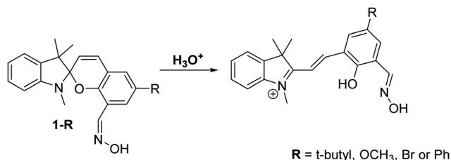
Scheme 3 Oxime-appended spirobenzopyrans 1-R for the use as pH fluorescent probes. Measurement conditions: HEPES/ACN (8:2) buffer solution.
