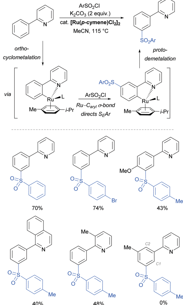
Fig. 11 (a) Pd-Catalysed ortho C–H sulfonation; (b) Ru-catalysed meta C–H sulfonation: proposed reaction mechanism and selected examples.
