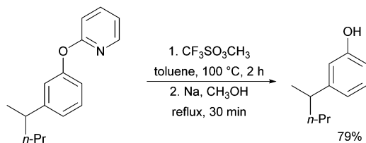
Scheme 13 Deprotection of phenols after alkylation.
