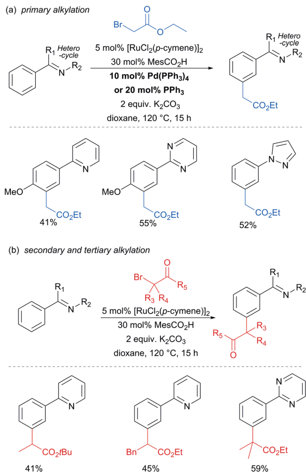
Fig. 25 meta -Alkylation with of \alpha -halocarbonyls.
