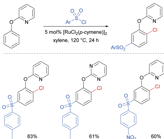
Fig. 21 Selected examples for dual ortho/meta selective functionalisation of 2-phenoxypyridines.
