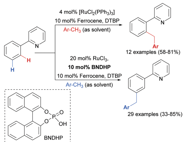
Scheme 15 ortho - and meta -Selective benzylation of 2-arylpyridines.
