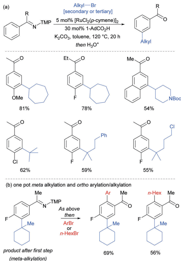
Fig. 26 (a) meta -Selective alkylation of ketimines (b) one-pot procedure for meta followed by ortho arylation/alkylation of ketimines; TMP = 3,4,5-trimethoxyphenyl.
