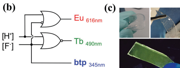
Fig. 24 (a) The truth table of the logic functions. a [H + ] = 2 mM; b [F - ] = 1 mM. (b) A circuit diagram of the observed logic gate functions. c Phosphorescence. d Fluorescence. (c) Images of Eu 13 and Tb 23 based gels when swelled in H 2 O (left) and CH 3 OH (right) under ambient light, after drying and irradiation at 254 nm, demonstrating the (0,0) state. Reproduced with small alterations from ref. 45 with permission from Royal Society of Chemistry, copyright 2015.
