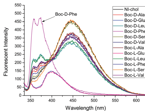
Fig. 2 Fluorescence changes of NI-chol 1 (10 \mu M ) in CH_3CN -DMSO (95:5, v/v) with D and L isomers of Ala, Glu, Leu, Phe, Ser and Val (500 \mu M ). ( \lambda_{ex} = 325 nm, slit 3 \times 5).
